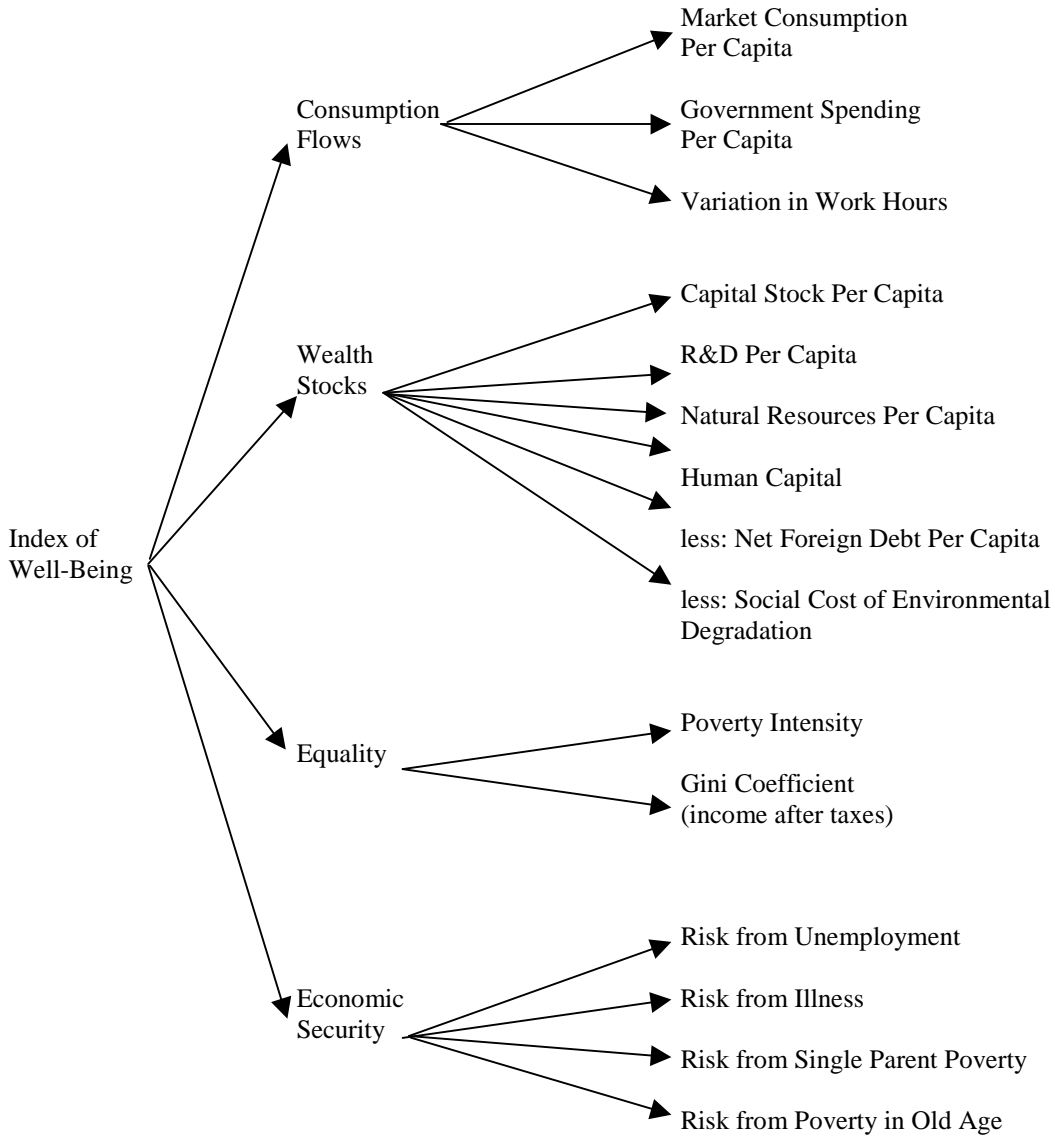
Figure 1: Weighting Tree
